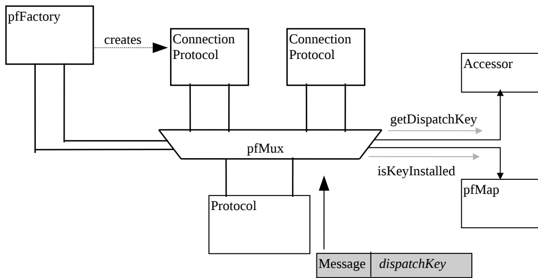
Multiplexer
