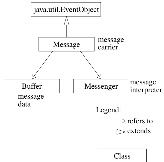
Figure 3: Structure of conduits messages
