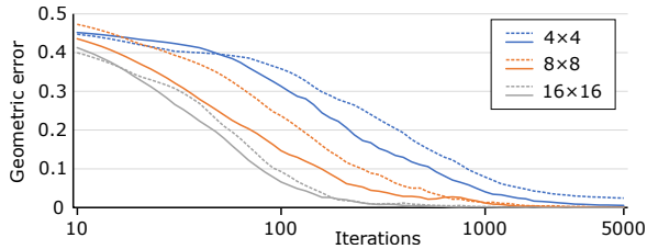
Fig. 5. Convergence of the cube shape and color optimization test (average of 10 successful optimizations). Vertical axis shows the average distance between vertices and their true positions in the unit cube. The solid curves indicate convergence in the continuous coloring mode (Figure 4), and the dashed curves correspond to the discontinuous coloring mode. As expected, the latter is somewhat more difficult to optimize. Note the logarithmic horizontal axis.
