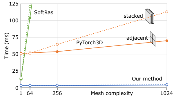
Fig. 9. The effect of geometric configuration on forward + gradient pass execution times in 1024 \times 1024 resolution. A 8 \times 8 grid base mesh (128 triangles) is repeated 1, 64, 256, or 1024 times (horizontal axis). The repeated meshes are either stacked in depth direction (dashed lines) or placed adjacent to each other on the same plane (solid lines). The meshes are scaled so that the output image always has the same number of pixels covered. PyTorch3D [Ravi et al. 2020] scales mostly with the total area of geometry, occluded or not, whereas our method is not slowed down by hidden geometry. SoftRas [Liu et al. 2019] has approximately constant cost per triangle, and cannot keep up with the other two methods.
