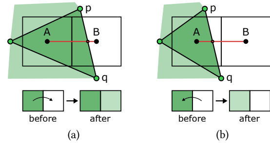
Fig. 3. Illustration of our analytic antialiasing method. A vertical silhouette edge p, q passes through centers of horizontally adjacent pixels A and B . This is detected by the pixels having a different triangle ID rasterized into them. Pixel pair A, B is processed together, and one of the following cases may occur. (a) The edge crosses the segment connecting pixel centers inside pixel B , causing color of A to blend into B . (b) The crossing happens inside pixel A , so blending is done in the opposite direction. To approximate the geometric coverage between surfaces, the blending factor is a linear function of the location of the crossing point — from zero at midpoint to 50% at pixel center. This antialiasing method is differentiable because the resulting pixel colors are continuous functions of positions of p and q .
