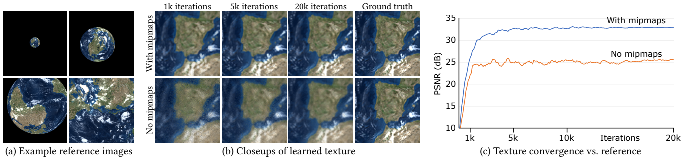
Fig. 6. Filtered texture sampling via mipmaps helps considerably when learning a texture in a difficult geometric setup. See text for full description. (a) Example synthetic reference images in 512 \times 512 resolution. (b) With mipmapping enabled, sampling is prefiltered and gradients are routed to the correct detail levels. Without mipmaps, faraway views yield badly filtered samples and spurious, noisy texture updates that do not converge to the correct solution. (c) Convergence of the learned texture compared to the reference texture. Learning rate schedule was optimized for the “no mipmaps” case, and the same schedule was used with mipmaps.
