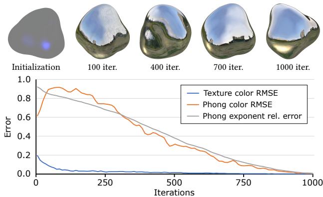
Fig. 7. Optimizing environment map texture and Phong BRDF parameters in a synthetic test case. Top: Example renderings at various iteration counts. The texture converges slightly unevenly due to the distribution of indirect texture lookups, as seen at 100 iterations. Bottom: Convergence of the learned parameters over the course of optimization.
