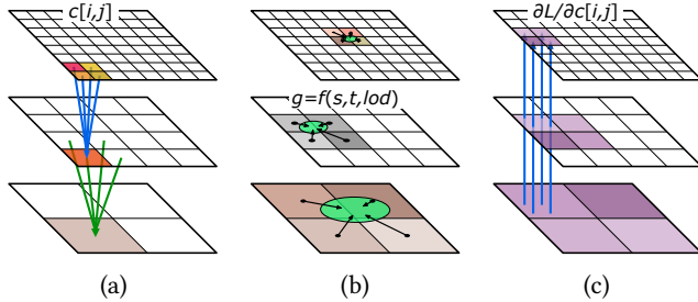
Fig. 2. Filtered differentiable texture lookup with a non-constant texture. (a) In the beginning of forward pass, prefiltered MIP levels c_{lod} are constructed from the full-resolution texture c[i, j] by repeated downsampling using a 2 \times 2 box filter. (b) In forward pass, each lookup g = f(s, t, lod) interpolates prefiltered values on the appropriate MIP level as determined by the size of sample footprint. In backward pass, we receive incoming gradients \partial L / \partial g . Texture coordinate gradients \partial L / \partial s and \partial L / \partial t for each lookup are computed based on these and contents of texels that were used in interpolation. Simultaneously, texture image gradients \partial L / \partial c_{lod}[i, j] are accumulated into each MIP level. In a trilinear lookup, these calculations are performed on two adjacent levels and weighted according to the fractional part of lod . (c) To produce outgoing full-resolution texture image gradients \partial L / \partial c[i, j] , we sum the accumulated gradients from all MIP levels.
