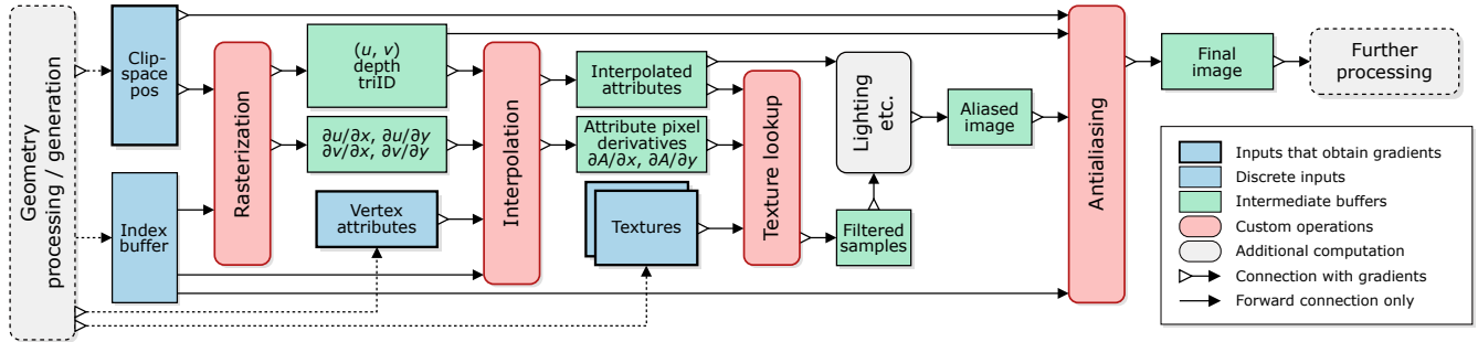
Fig. 1. A simple differentiable rendering pipeline with our proposed primitive operations highlighted in red. The input data for rendering (blue) may be generated by, e.g., a neural network if the pipeline is part of a larger computation graph. In simpler setups the geometry processing might include only the model/view/perspective transformations for vertex positions with other inputs being constants or learnable parameters. All intermediate buffers (green) are in image space. Connections with gradients are denoted by a white triangle. Channel counts are fixed only for vertex positions and indices, and in the intermediate buffers produced by the rasterization operation. There are no restrictions on the channel counts for vertex attributes, textures, related intermediate data, or the output image.
