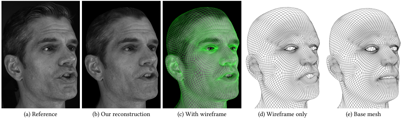
Fig. 10. An example frame from the reconstruction of a 89-frame sequence. (a) One of the 9 camera images for the frame. (b–d) Our reconstructed texture and geometry, rendered from the same viewpoint using the known camera parameters. (e) Base mesh V_{base} used as the starting point for optimization.
