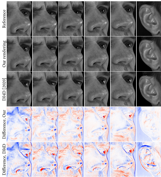
Fig. 11. Closeup of the nose reveals significant motion and deformation. Our solution reproduces the changes in geometry faithfully, while the solution from DI4D [2020] severely attenuates the deformations. False-color difference images (red/blue = brighter/darker than reference) highlight the geometric discrepancies around the nostrils. In our solution, the geometric silhouettes are located correctly and the differences are only due to defocus blur in the reference images that is lacking in our renderings. Right: The DI4D solution did not attempt to recover the motion of ears. We placed no constraints on which vertices are allowed to move during optimization, and thus also captured this motion.
