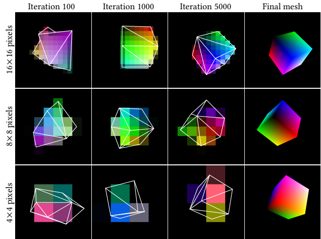
Fig. 4. To validate that our visibility gradients provide useful information even for small triangles, we infer vertex positions and colors of a simple mesh in extremely small resolutions. The geometry of the current solution is superimposed on the rasterized images for illustration purposes only. Right-most column shows the final, optimized mesh rendered in high resolution. In 4 \times 4 resolution, the average triangle area is only 0.54 pixels. The optimization nonetheless converges to the correct solution, albeit slower than in higher resolutions. In 2 \times 2 resolution the optimization fails to converge.
