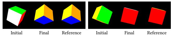
Fig. 8. Two example cases from the cube pose optimization test. With trivial noise-based regularization, we obtain an average error of 48.62^\circ which is an improvement over the 63.57^\circ of Liu et al. [2019], indicating that the blur and transparency offered by SoftRas are not necessary in this task. The average error is dominated by local minima where the pose looks correct but the colors are wrong (see example on the right with \sim 180^\circ final pose error – the yellow face should be on top instead of white). Customizing the optimization method to suit the task better lowers the average error to 2.61^\circ . Some cases are impossible due to only one face of the cube being visible in the reference image, but they are rare enough to not contribute significantly to the averages.
